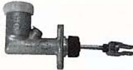
Master cylinder, Lucas Girling style with 3/4" bore
