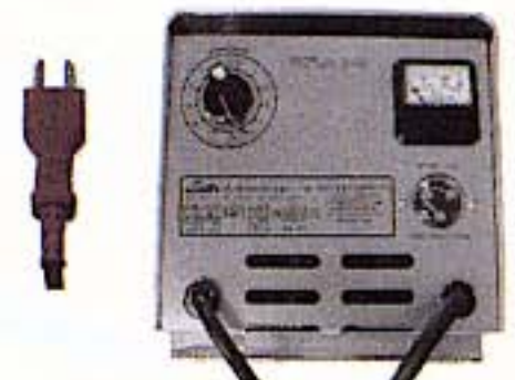
Manual timer charger with 2 prong Lester molded plug
