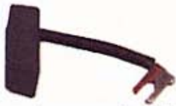
Brush set with spring groove for GE motors. 1-7/16" L x 5/8" W x 1/2" D
