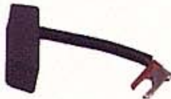
Brush set with spring groove For GE® motors. 1-7/16" L x 5/8" W x 1/2" D
